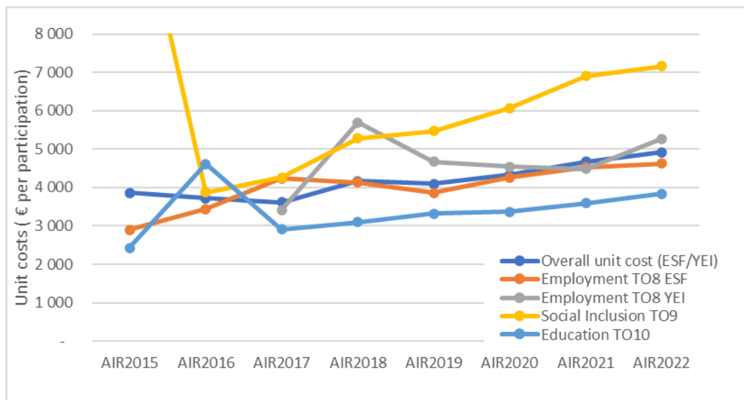
Figure 17. Trend in cost per individual immediate result
